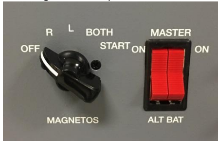
Image 45: Switch Panel 1 Starter Switch*
